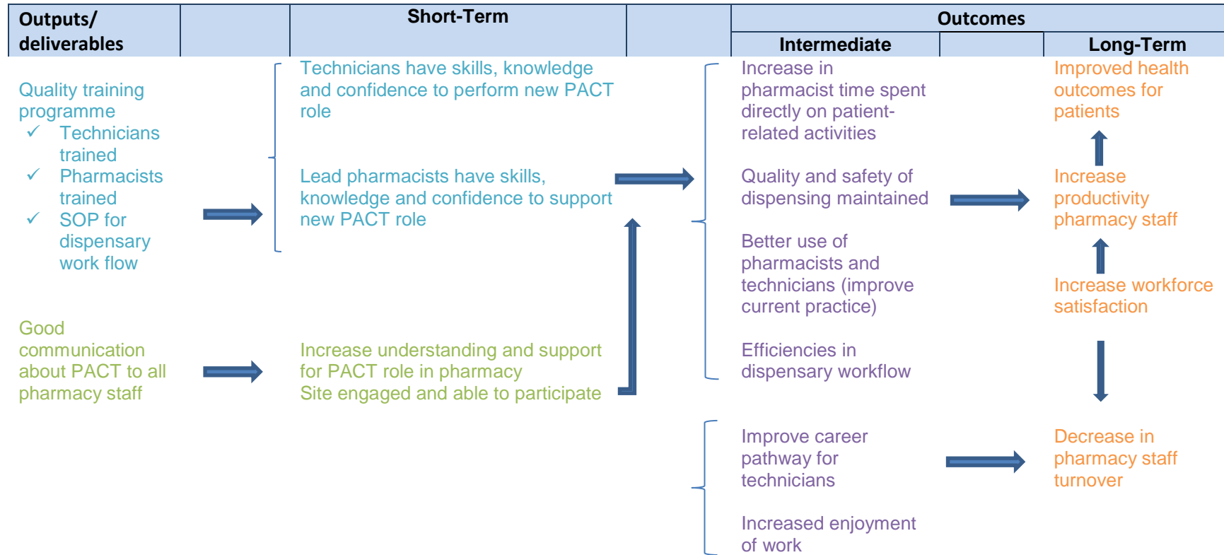
Figure 1: Project logic
